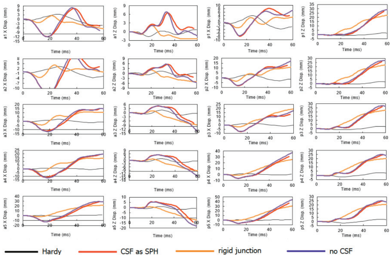
Fig. 8. Benchmark aHEAD simulation (CSF as SPH) with two modified head models: "rigid junction" and "no CSF". The displacements are compared with Hardy C755-T2 test results
