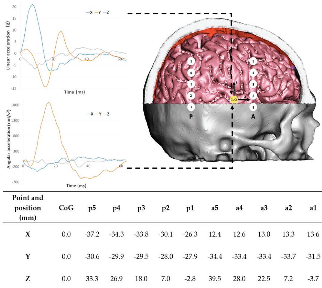
Fig. 4. Boundary conditions for a C755-T2 Hardy test, points a1–a5 refer to the anterior, and the p1–p5 points to posterior [25]
