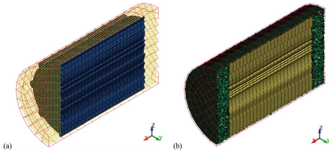
Fig. 6. Cross-section of modelled container including liquid fluid and gelatine insert: (a) model with SPH, (b) model with TET10 finite elements
