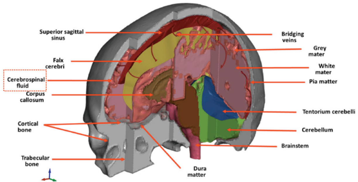
Fig. 3. aHEAD benchmark model, developed by authors [25]. The further modified cerebrospinal fluid is indicated in a dashed frame
