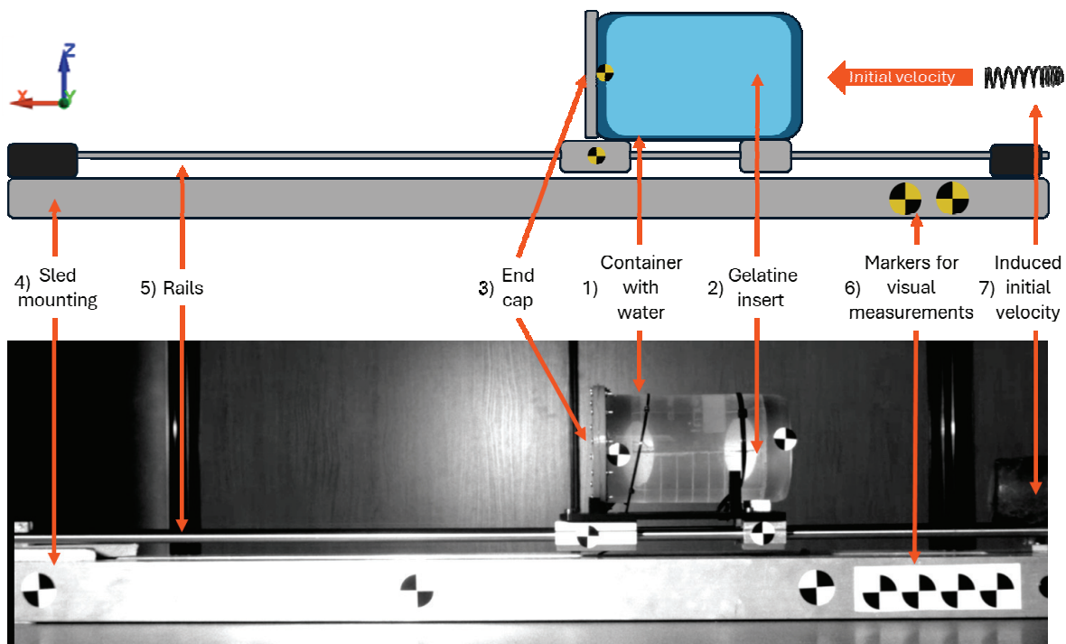
Fig. 5. The sledge experimental setup for gelatine insert measurements
