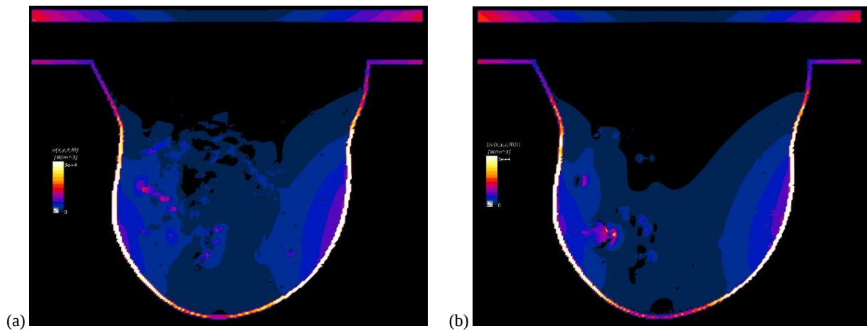
Fig. 4. Eddy currents power losses in xz -plane in the case of female breast model: (a) without tumor and (b) with tumor after the 25-min magnetic hyperthermia treatment
