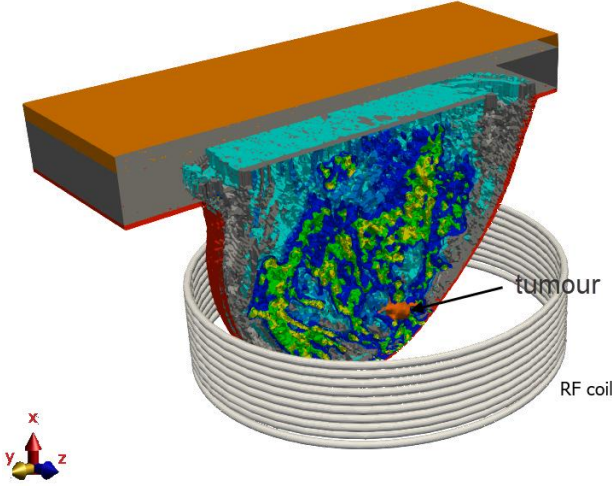
Fig. 2. Model of the 3D female breast phantom including naturalistic tumor and RF coil
