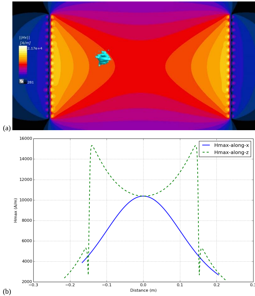
Fig. 3. Magnetic field strength distributions inside the 10-turn RF coil: (a) spatial distribution on the xy -plane and (b) H_{\max} curves along the x -axis (blue) and z -axis (green)
