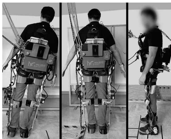
Fig. 2. Examples of the subject-exoskeleton setup positions in the measurement station.
