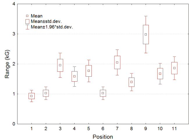
Fig. 5. Mean intra-individual ranges (|maximal – minimal value| from 10 consecutive trials performed in each position, each vector direction and in each individual) and standard deviations of the forces causing falls in consecutive test positions and [vector directions]: 1 – 2-leg standing [posterior], 2 – 2-leg standing [anterior], 3 – 2-leg standing [lateral (right)], 4 – 1-leg standing (right leg supporting) [posterior], 5 – 1-leg standing (right leg supporting) [anterior], 6 – 1-leg standing (right leg supporting) [lateral right], 7 – 1-leg standing (right leg supporting) [lateral left], 8 – step (right leg swinging) [posterior], 9 – step (right leg swinging) [anterior], 10 – step (right leg swinging) [lateral right], 11 – step (right leg swinging) [lateral left]
