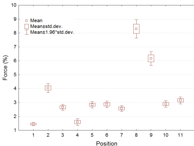
Fig. 4. Mean relative values (normalized for the body plus exoskeleton weight) and standard deviations of the forces causing falls in consecutive test positions and [vector directions]:
