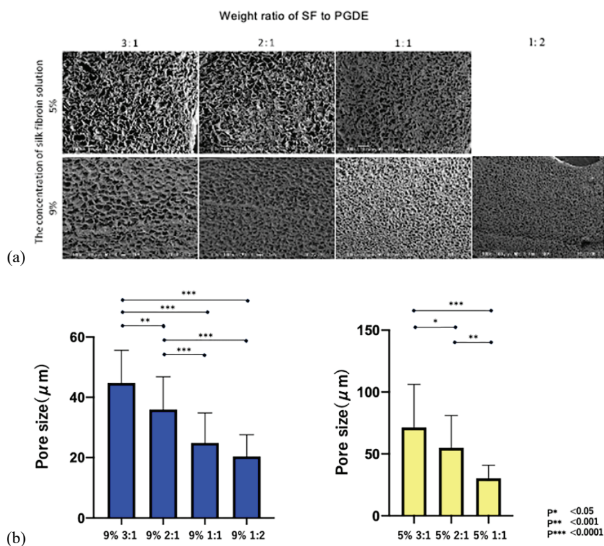
Fig. 2. (a) SEM images of poly(ethylene glycol diglycidyl ether) (PGDE)/silk fibroin (SF) sponge cross-sections, showing the weight ratio of SF to PGDE, (b) histograms of the pore size distribution in SF/PGDE sponges
