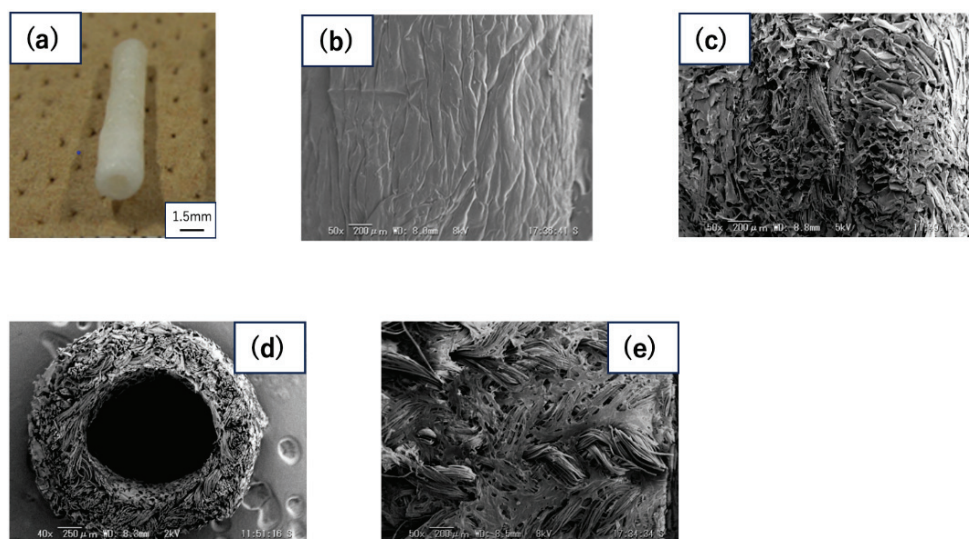
Fig. 3. (a) Macroscopic view of porous silk vascular graft (PSVG) and SEM images of (b) the outer surface immediately after fabrication, (c) the outer surface after peeling off the surface with cellophane tape, (d) the graft cross-section, and (e) the graft inner surface
