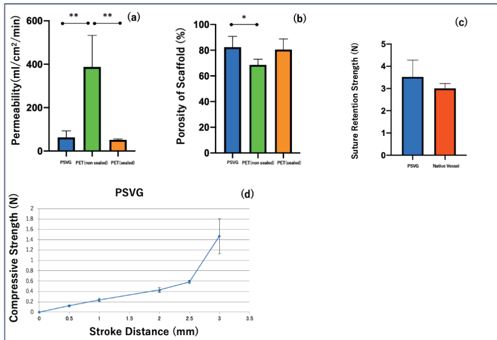
Fig. 4. (a) Permeability, (b) porosity of porous silk vascular graft (PSVG) and gelatin-sealed and non-sealed polyethylene terephthalate (PET) grafts, (c) suture retention strength of PSVG and native vessels. P^* < 0.05 , P^{**} < 0.01 , (d) the progression of compressive strength (N) of the PSVG when compressed to 3 mm
