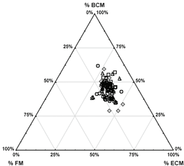
Fig. 1. Distribution of players in the system of three variables of body composition (○ – football, Δ – basketball, □ – handball, ◇ – volleyball)
