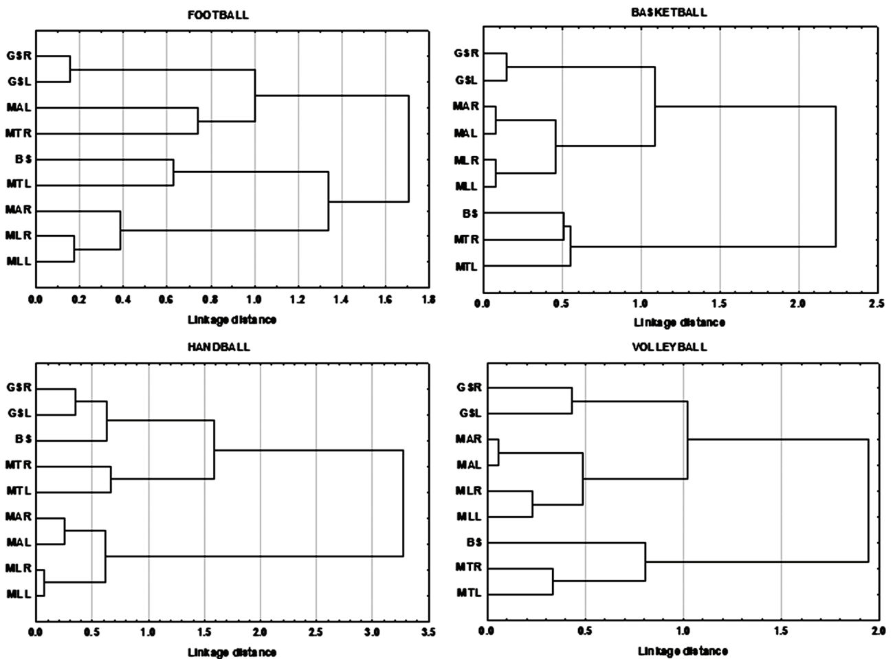
Fig. 2. Cluster analysis of musculature of body segments and strength in football, basketball, handball, and volleyball athletes. BS – back strength, GSL – grip strength left, GSR – grip strength right, MAL – muscle arm left, MAR – muscle arm right, MLL – muscle leg left, MLR – muscle leg right, MTL – muscle trunk left, MTR – muscle trunk right
