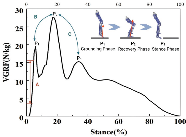
Fig. 4. Loading rate (P1 – first peak, P2 – second peak, P3 – third peak, A – the first vertical peak loading rate, B – the time difference from the first peak to the second peak, C – the time difference from the second peak to the third peak)
