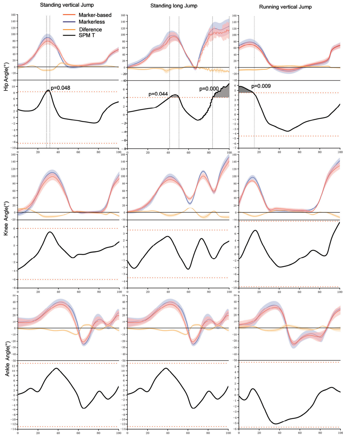
Fig. 3. Rows 1, 3 and 5: the aggregate curves of lower limb joint Angle differences between 12 participants who completed standing vertical jump, standing long jump and running vertical jump with marked and unmarked motion capture systems. The second, fourth, and sixth rows of figures corresponding to 1, 3 and 5: the analysis results of SPM paired T -test, where the horizontal red dotted line represents the critical random field theoretical threshold of the significance level ( p < 0.05 ), and the dashed rectangle represents the significant region.
