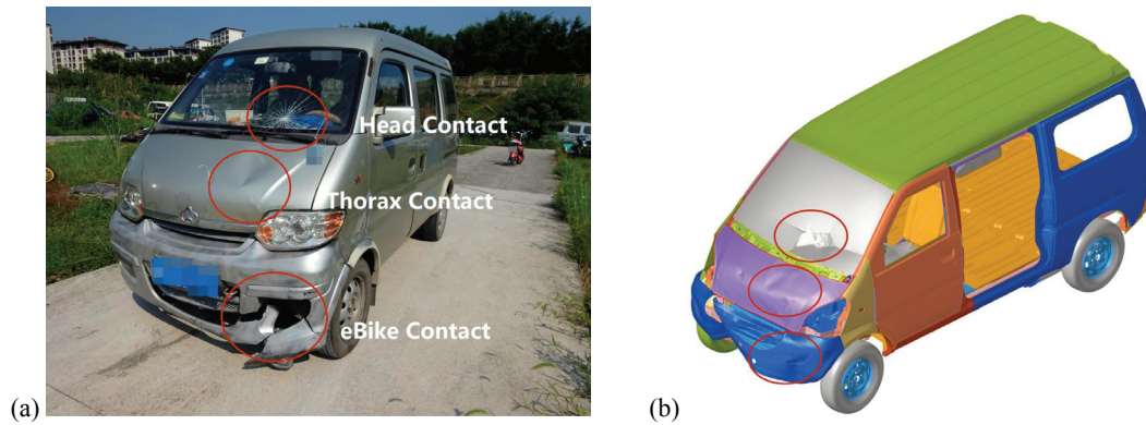
Fig. 9. Comparison of collision traces: (a) accident vehicle trace, (b) simulating collision trace
