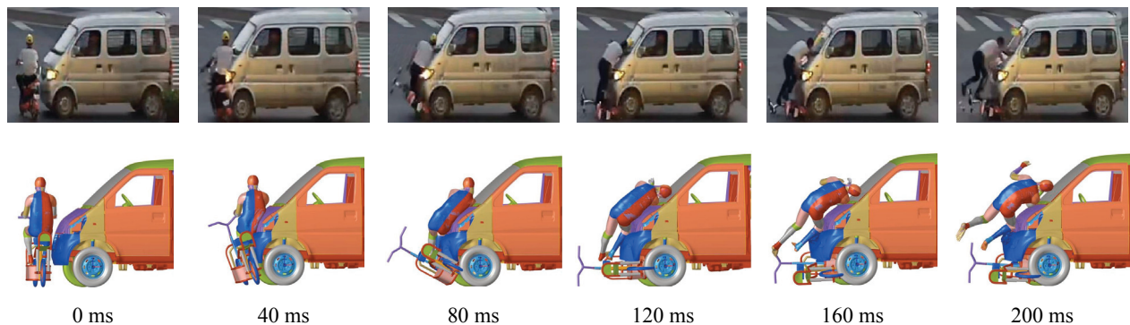
Fig. 8. Comparison of accident video and reconstruction results
