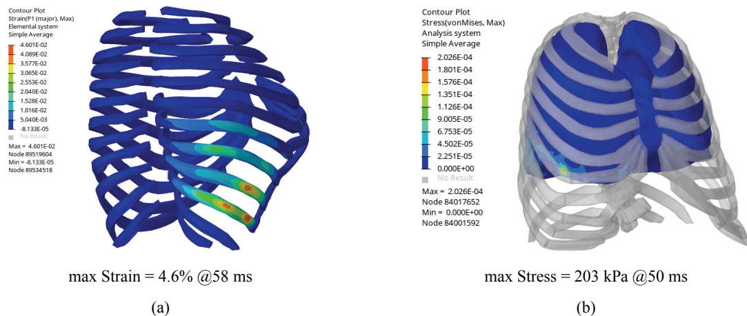
Fig. 10. Thorax injury situation: (a) rib strain, (b) lung stress
