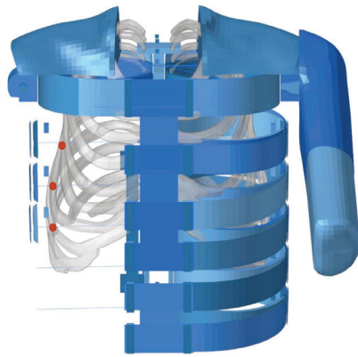
Fig. 16. Comparison of WorldSID thorax module measurement points and THUMS rib deflection measurement points
