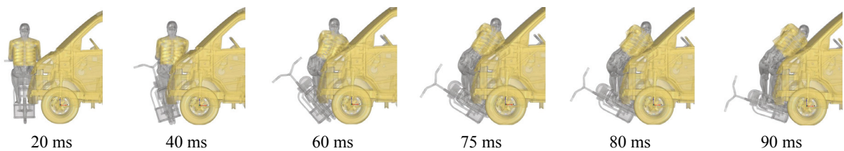
Fig. 14. Comparison of WorldSID thorax module and THUMS motion (with the added abdominal mass)
