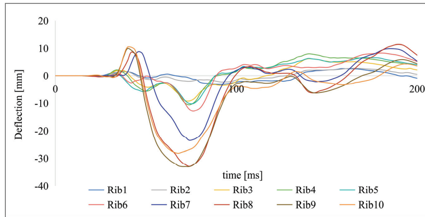
Fig. 12. THUMS rib outermost deflection
