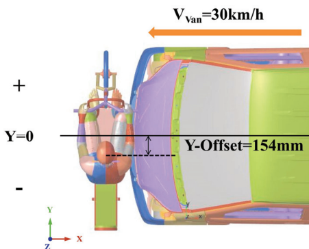
Fig. 5. Definition of vehicle Y-Offset and velocity
