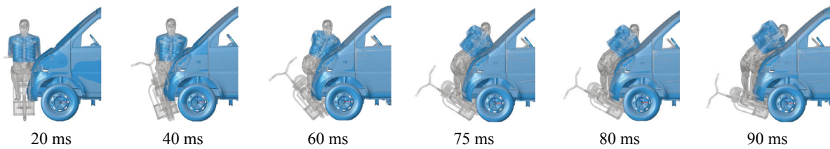
Fig. 13. Comparison of WorldSID thorax module and THUMS motion (without the added abdominal mass)
