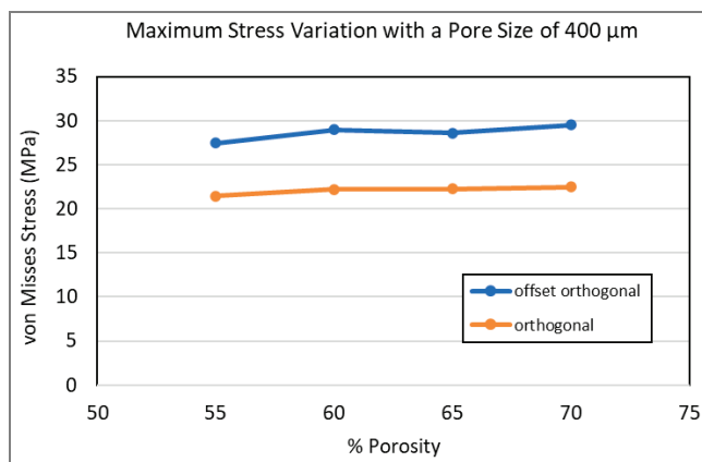
Fig. 5. Maximum von Mises stress variation for a pore size of 400 µm and different porosities. The behavior of orthogonal geometry and offset orthogonal geometry is illustrated
