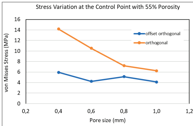
Fig. 8. Stress variation at the control point for a fixed porosity of 55% and different pore sizes. The behavior of orthogonal geometry and offset orthogonal geometry is illustrated
