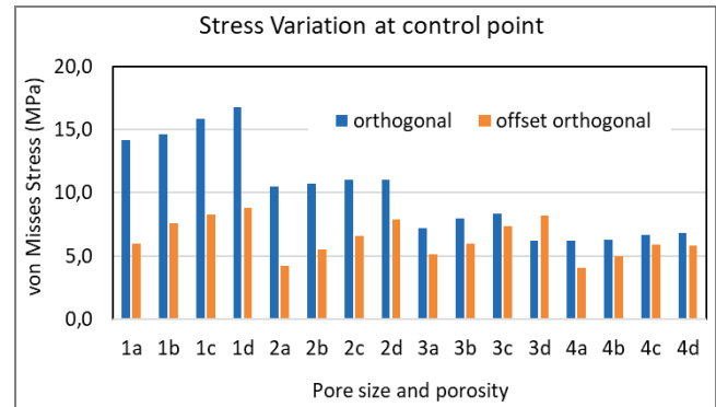
Fig. 9. Stress variation at control points for orthogonal and offset orthogonal geometries
