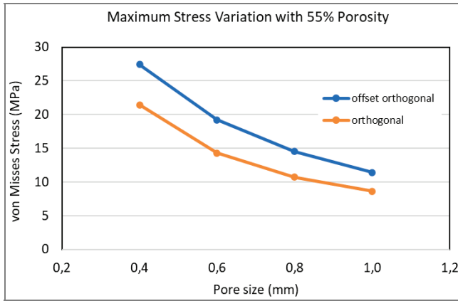
Fig. 7. Maximum stress variation for a fixed porosity of 55% and different pore sizes. The behavior of orthogonal geometry and offset orthogonal geometry is illustrated
