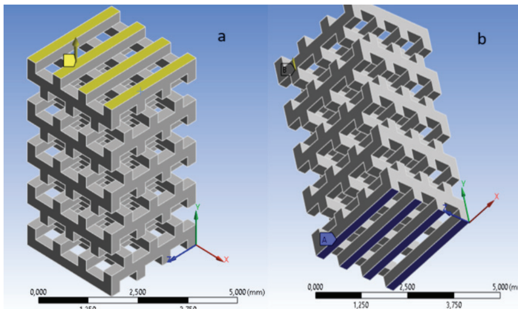
Fig. 3. Boundary condition configuration for the simulation: (a) imposed displacement, (b) fixed support
