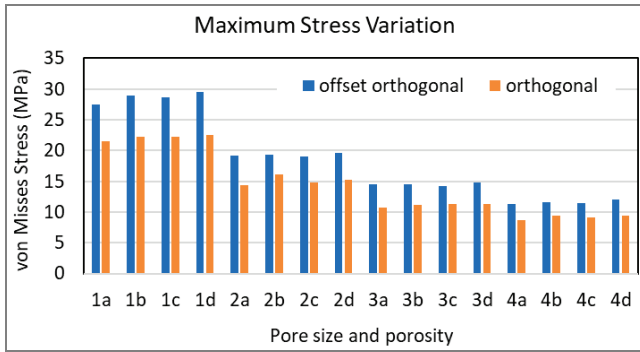
Fig. 10. Variation of maximum stresses for orthogonal and offset orthogonal geometries
