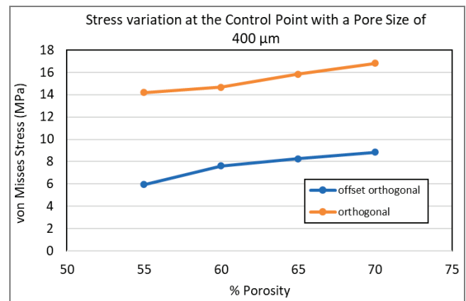
Fig. 6. Stress variation at the control point for a pore size of 400 µm and different porosities. The behavior of orthogonal geometry and offset orthogonal geometry is illustrated
