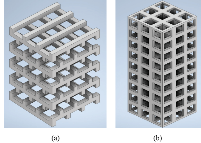
Fig. 2. Offset orthogonal structures (a) and orthogonal structures (b)
