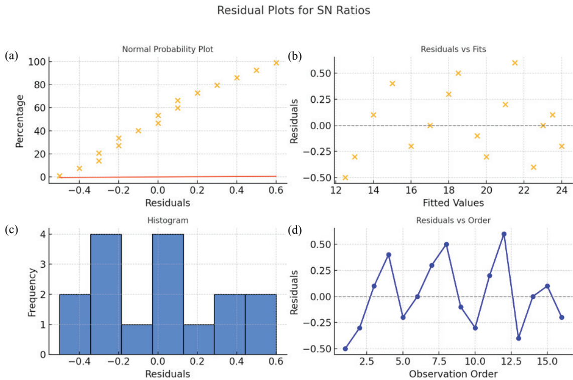
Fig. 12. Residual plots for S/N ratios
