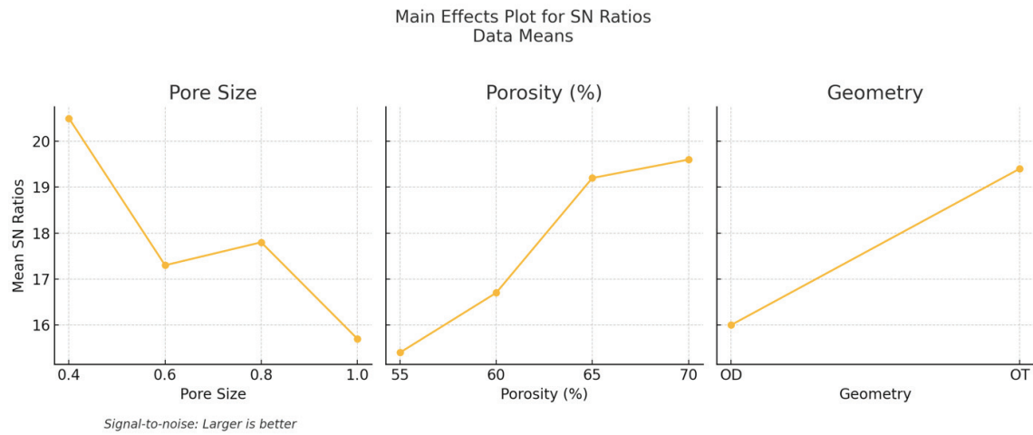
Fig. 11. Main effects plots for S/N ratios
