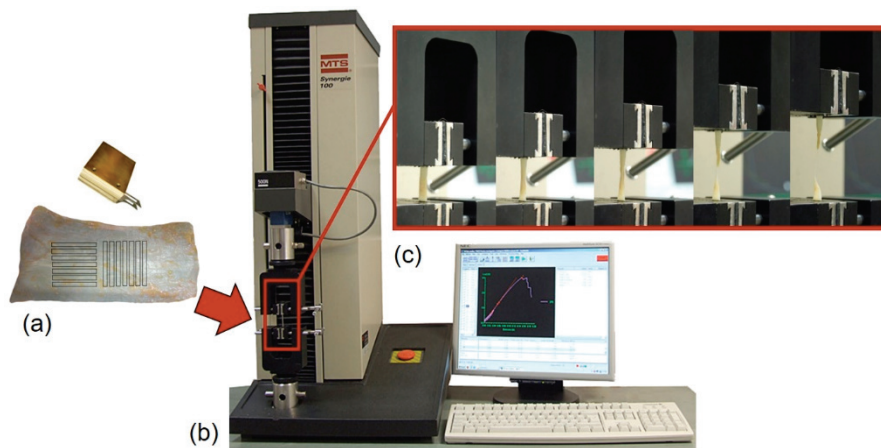
Fig. 1. Specimen of human fascia lata with visible lines of samples cutting (in two directions: longitudinal and transversal to the direction of collagen bundles arrangement) using a punch (a), the experimental setup – testing machine MTS Synergie 100 (b), fascia's specimen fixed in the clamp was subjected to a controlled tension until failure (c)
