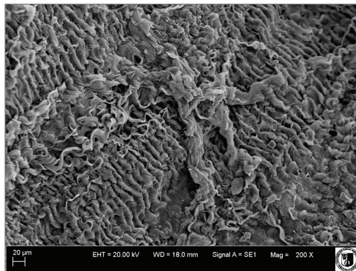
Fig. 8. SEM image of the human fascia lata; collagen bundles exhibiting evident undulation appearance (crimped collagen pattern) (mag. 200×)
