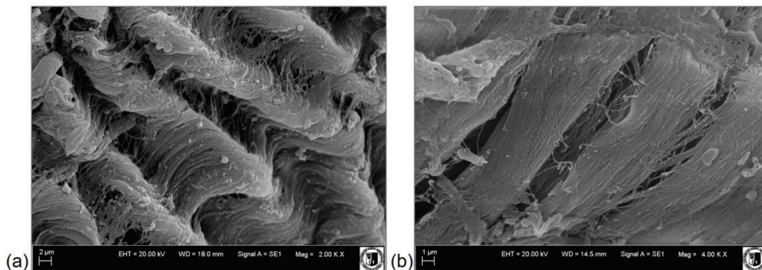
Fig. 9. SEM images of human fascia lata before (a) (mag. 2000×), and after uniaxial tensile test (b) (mag. 4000×)
