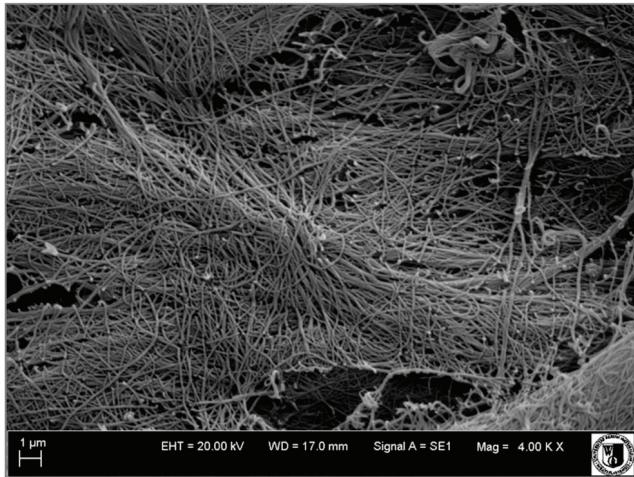
Fig. 10. SEM images of human fascia lata after tensile test; note fragmentation and rupture of individual collagen fibres (mag. 4000×)
