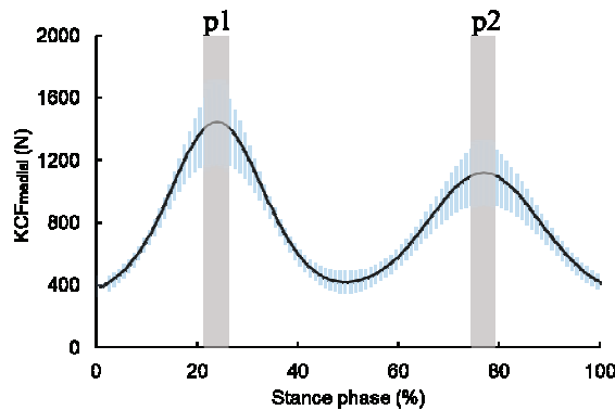
Fig. 3. Time profiles of Knee contact force on the medial compartment. Averaged across subject data are shown with standard deviation shades from initial contact (0%) to toe off (100%) of the more affected side.
