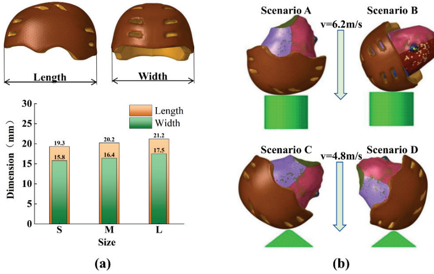
Fig. 3. (a) the dimensions of the helmets in different sizes, (b) the impact scenarios
