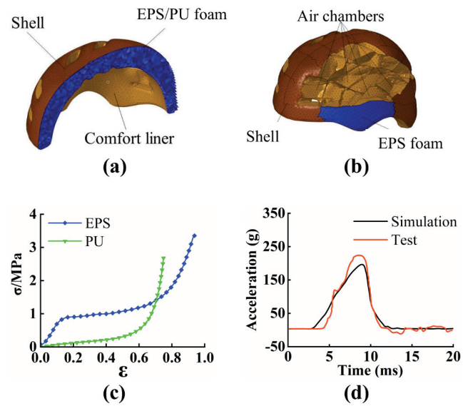
Fig. 2. The FE models of (a) the EPS/PU and (b) airbag helmet, (c) the stress-strain curves of EPS and PU material, and (d) the validation result of the EPS helmet model
