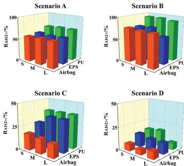
Fig. 7. The calculated AIS2+ brain injury risk of all impact simulations
