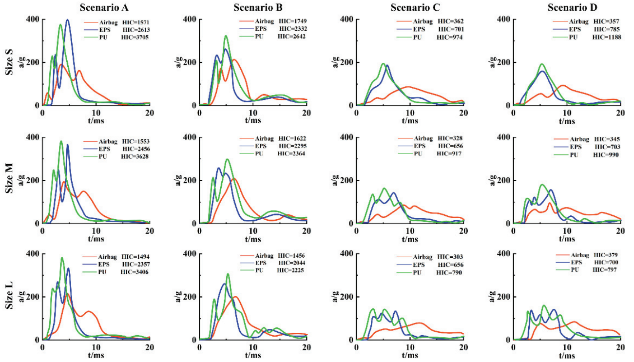
Fig. 4. The predicted head linear acceleration curves and HIC values of all impact simulations
