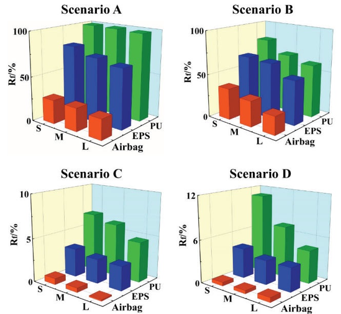
Fig. 5. The calculated skull fracture risk of all impact simulations
