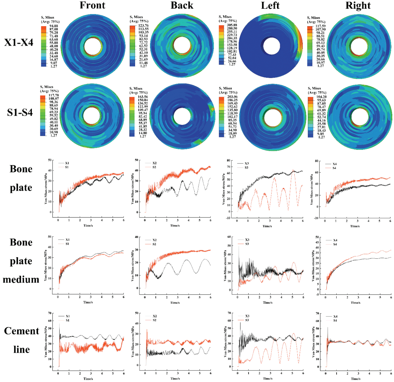
Fig. 7. Plot of the results of the kinetic analysis of the mesoscopic bone unit
