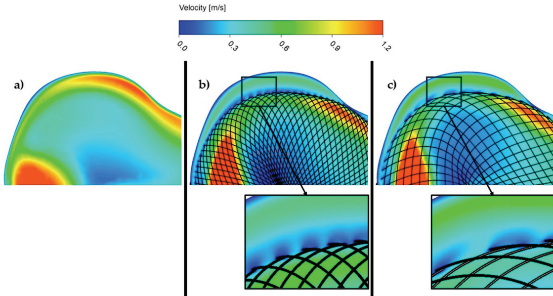
Fig. 2. Blood velocity distribution at a random control surface: (a) reference geometry (no stent), (b) stent \varnothing 4.5 mm; (c) stent \varnothing 6.0 mm
