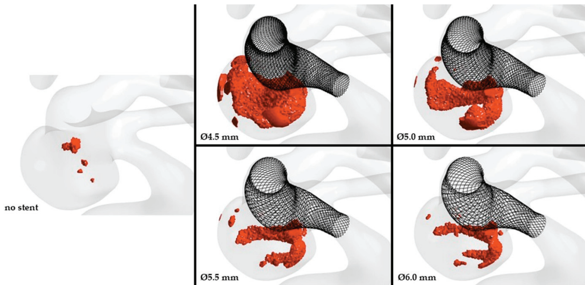
Fig. 5. Qualitative comparison of RVVB parameter inside the aneurysm dome
