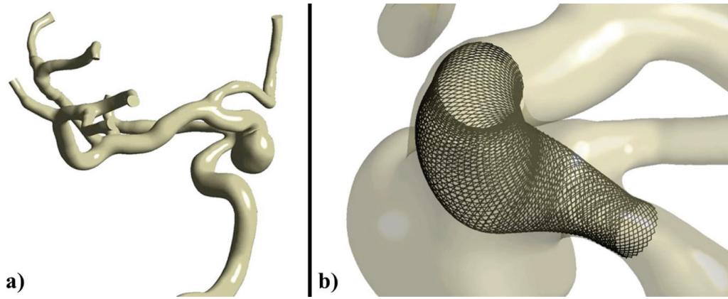
Fig. 1. Virtual models used in this research: (a) fragment of the patient-specific arterial tree network, (b) FD stent ( \varnothing 4.5 mm) implanted in the parent artery
