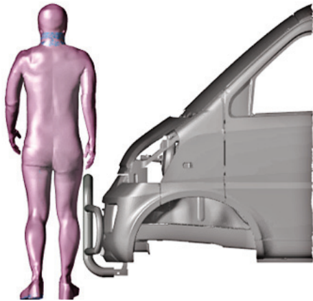
Fig. 6. Initial collision position of the analytical model
