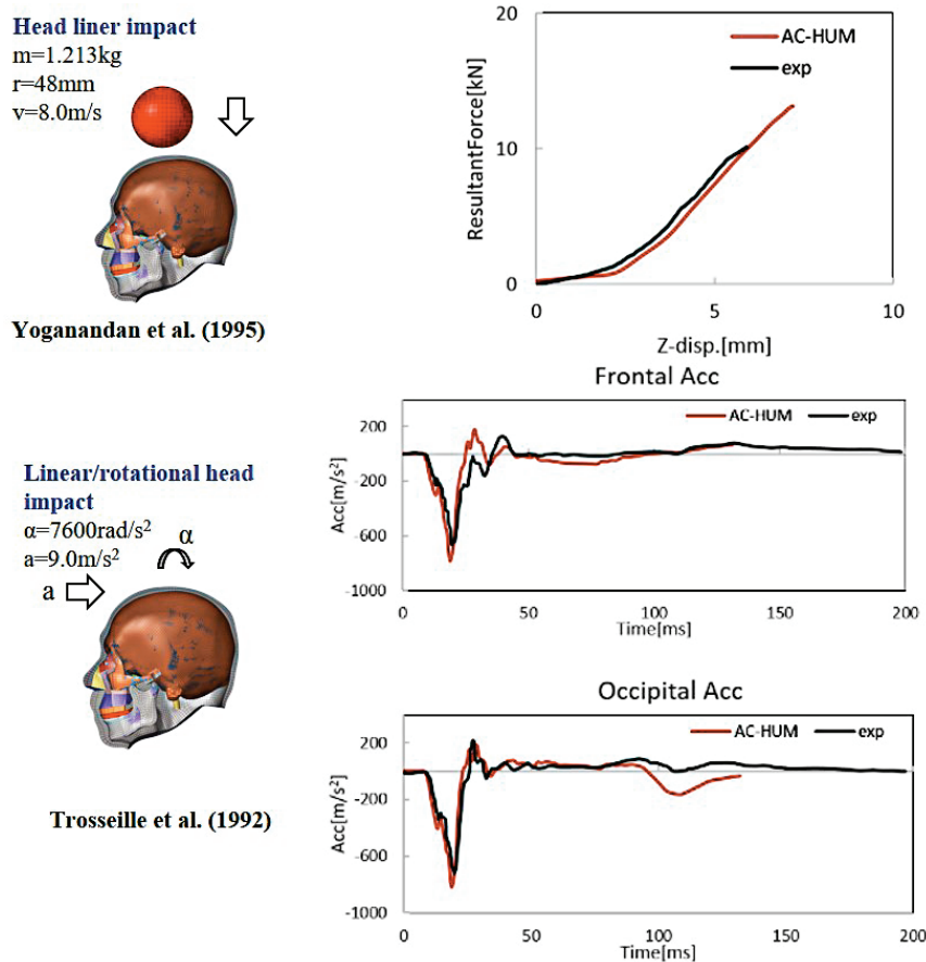
Fig. 3. Part verification of AC-HUMs head model
