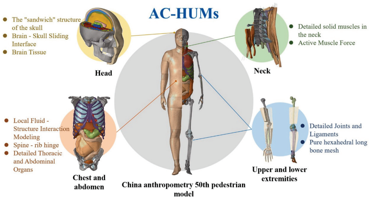
Fig. 2. AC-HUMs M50 pedestrian model
