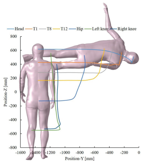
Fig. 8. Initial and final position of pedestrian model relative to minivan during collision
