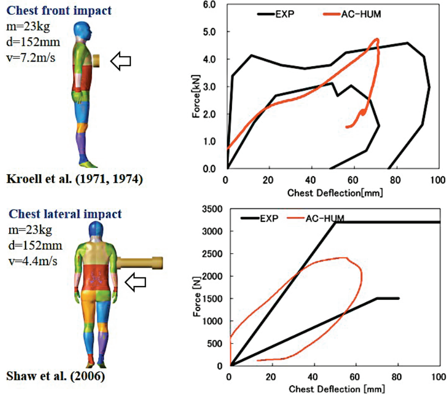
Fig. 4. Part verification of AC-HUMs chest model
