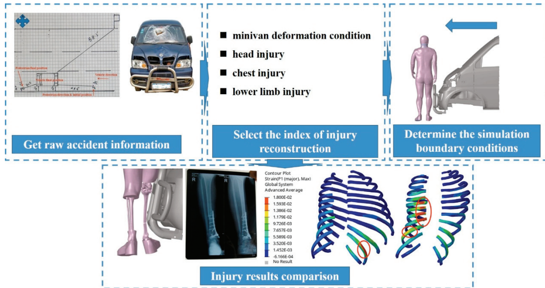
Fig. 1. Numerical reconstruction process based on real accident
