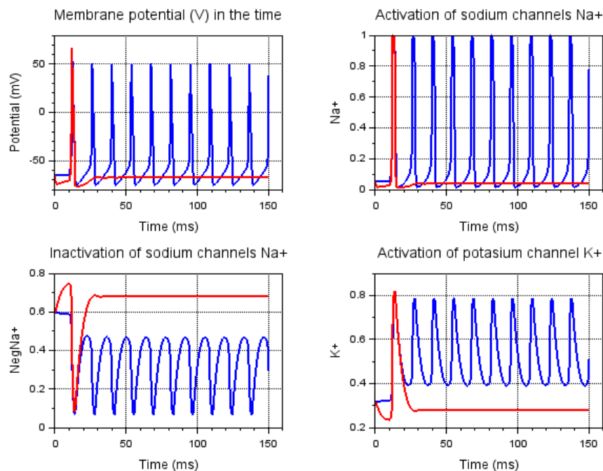
Fig. 4. Action potential for hyperconductivity of \text{Na}^+ and \text{K}^+ channels
