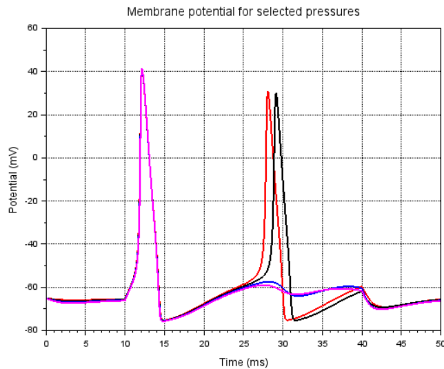
Fig. 5. Signal disturbances generated in the neural cell caused by a pressure pulse
