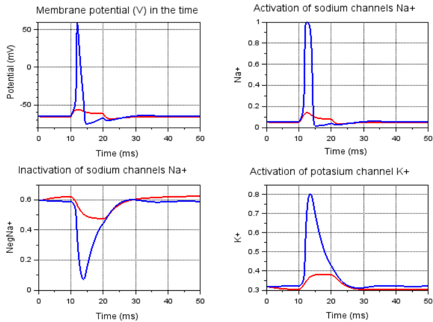
Fig. 3. Action potential for 10% conductivity of \text{Na}^+ and \text{K}^+ channel: blue line – 100% of conductivity, red line – 10% of conductivity
