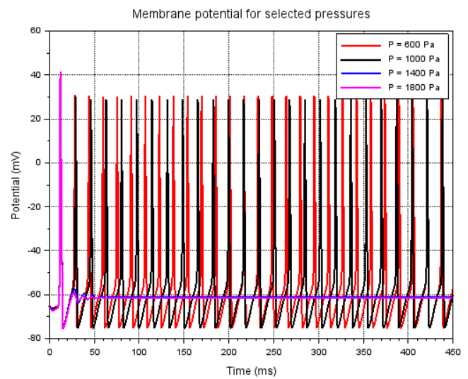
Fig. 6. Signal disturbances generated in the neural cell for selected pressure impulse
