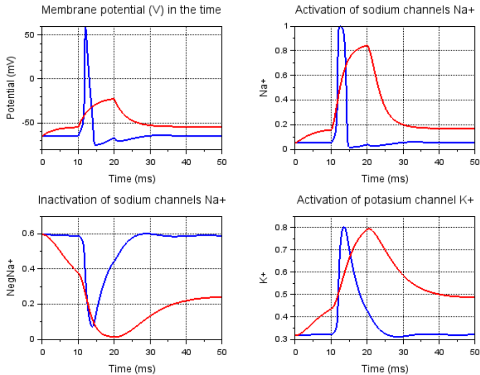
Fig. 2. Action potential for 50% conductivity of \text{Na}^+ and \text{K}^+ channel: blue line – 100% of conductivity, red line – 50% of conductivity
