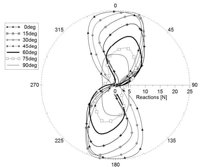
Fig. 10. Reaction forces in model M1, extortion “c”, Dyna Mesh
