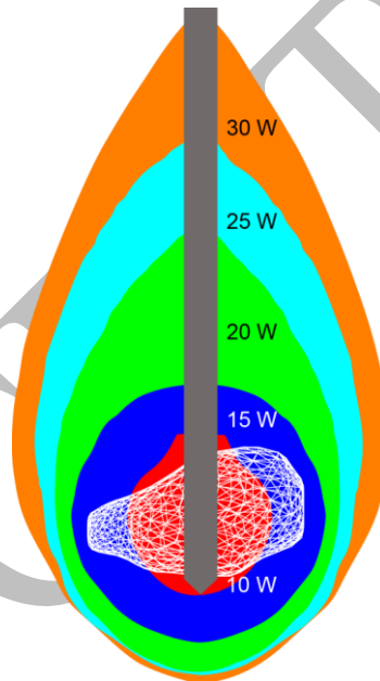
Figure 3. Isocontours composed of the totally ablated region (solid surface) after 600 s of MWA of tumor 1.04 [30] (triangulated surface) for input power from 10W to 30 W.
