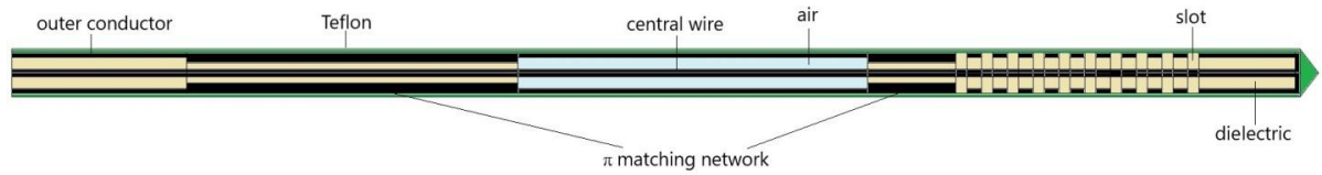
Figure 1. Schematic representation of a 10-slot antenna with a finely tuned impedance \pi -matching network to preserve surrounding healthy tissues. The distance between the two slots is 0.8 mm, while the width of the single slot is 0.6 mm.
