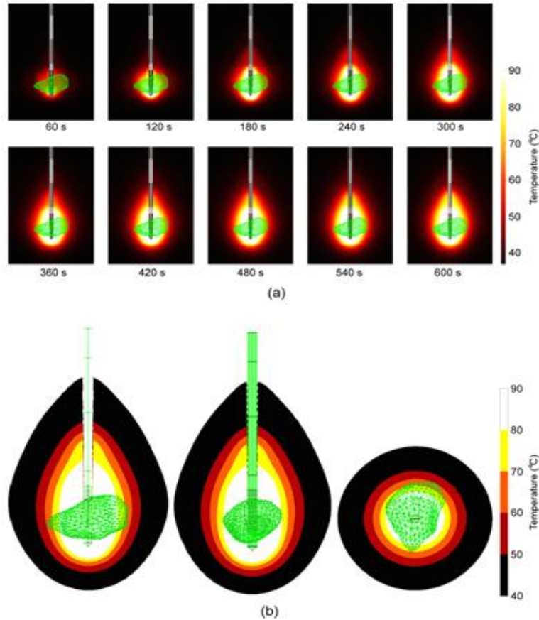
Figure 6. a) The time evolution of temperature distribution from 60s to 600s, and b) temperature distribution at different cross-sections at 600 s, around liver tumor 1.04 [30] (triangulated surface) during MWA at 2.45 GHz and the input power of 20 W.
