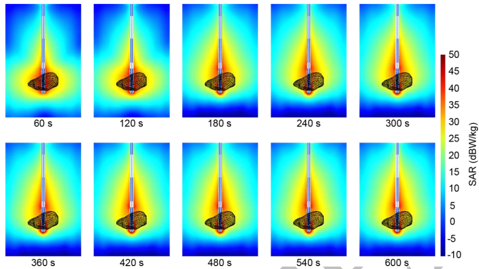
Figure 5. a) Time evolution of SAR distribution from 60 s to 600 s, and b) SAR distribution at different cross-sections at 600 s, around liver tumor 1.04 [30] (triangulated surface) during MWA at 2.45 GHz and input power of 20 W.
