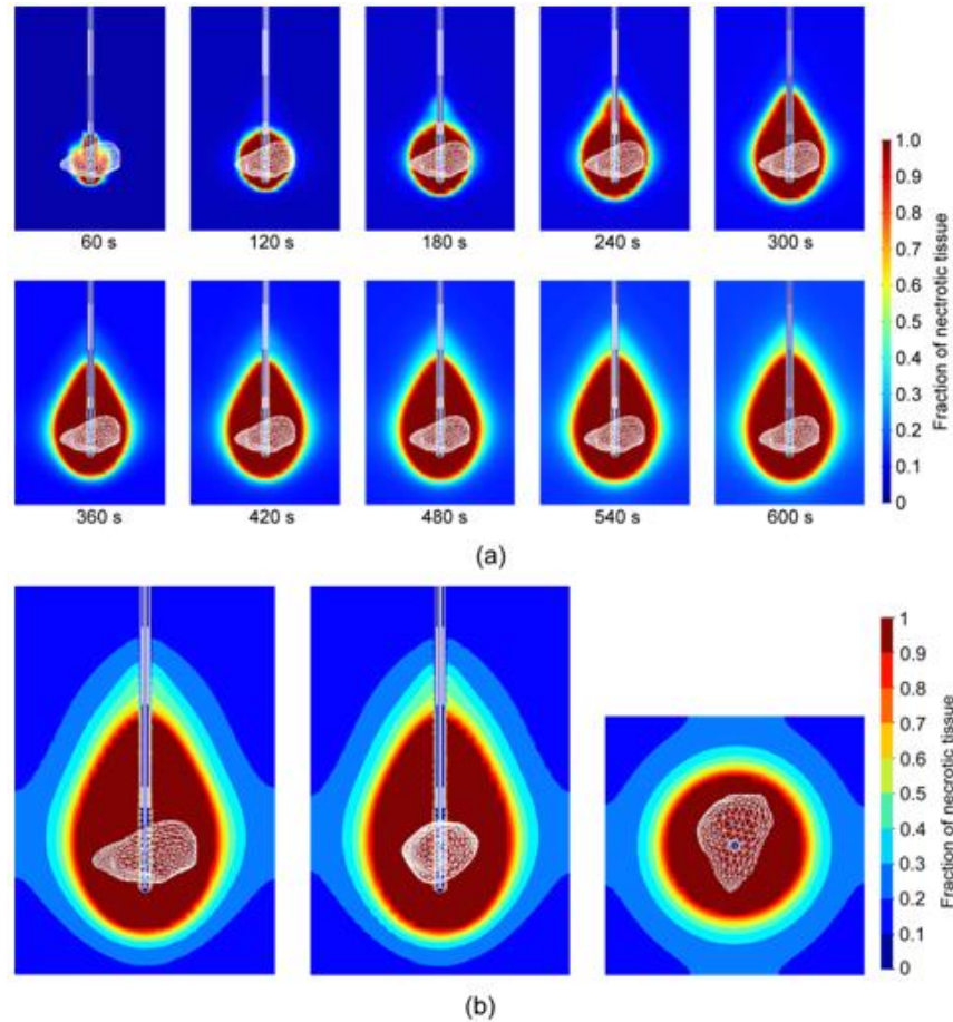
Figure 4. a) Time evolution of the fraction of necrosis from 60 s to 600 s, and b) fraction of necrotic tissue at different cross-sections at 600 s, around liver tumor 1.04 [30] (triangulated surface) during MWA at 2.45 GHz and input power of 20 W.
