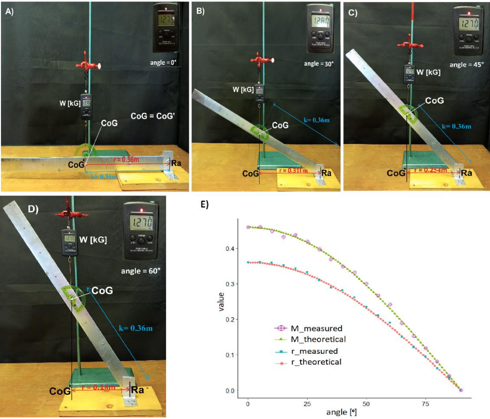
Figure 3. The result of measurements of the force of gravity ( W ) and the force arm ( r ) at different angles of inclination of a metal flat bar. A) horizontal positioning of the flat bar, the maximum value of the arm of gravity r=0.36\text{m} , gravity force W=1.275\text{kG} , B) at an angle of 30^\circ to the ground, r=0.31\text{m} , W=1.280\text{kG} , C) at an angle of 45^\circ to the ground, r=0.261\text{m} , W=1.270\text{kG} , D) at an angle of 60^\circ from the ground, r=0.19\text{m} , W=1.270\text{kG} , E) Dependence of the torque values and the force arm on the flat bar inclination angle from 0^\circ to 90^\circ .
