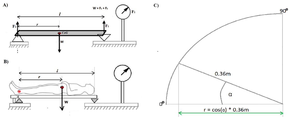
Figure 1. Determining the centre of gravity of the CoG using the one-sided lever method. A) A metal flat bar (grey) placed in a horizontal position enabling measurement of the reaction force. r – arm of the force, l – length of the lever, W – weight of the flat bar, F_1 – reaction force at the fulcrum on the scale, F_2 – reaction force at the rotation point (support point of the one-sided lever). B) Determining the centre of gravity for a human body tilting on the trochlea of the talus. The fulcrum for the one-sided lever is located on the axis of the upper ankle joint (red circle with a cross). The weight of the foot is not included in the body weight because it provides a support platform for the tilting body. C) Method of calculating the force arm ( r ) with a known angle of inclination and distance from the axis of rotation to the center flat bar gravity (CoG).
