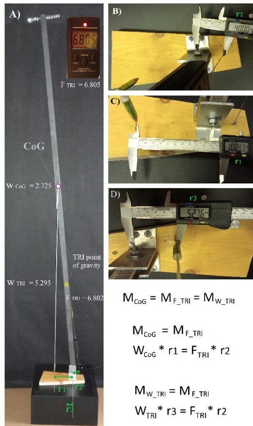
Figure 5. An example of balancing the moment of gravity of a tilted metal flat bar with the moment of the "triceps calf muscle" is presented in the model. A) Measuring system for simulating gravitational and muscle torques. CoG - the centre of gravity of the flat bar (55% of the distance from the ground), TRI point of gravity - a point halfway between the CoG and the ground (simulates the "proximal insert of the triceps surae muscle), W_{CoG} - the weight of the tilted flat bar at the centre of gravity, W_{TRI} - the weight of the tilted flat bar at the TRI point of gravity, F_{TRI} - the force of the triceps calf muscle balancing the moment of gravity at the CoG point ( M_{CoG} ) and in the TRI point of gravity ( M_{W\_TRI} ), B) distance of the TRI action line from the axis of rotation ( r_2 ), C) measurement of the arm of gravity for CoG ( r_1 ), D) measurement of the arm of gravity for TRI point of gravity ( r_3 ).
