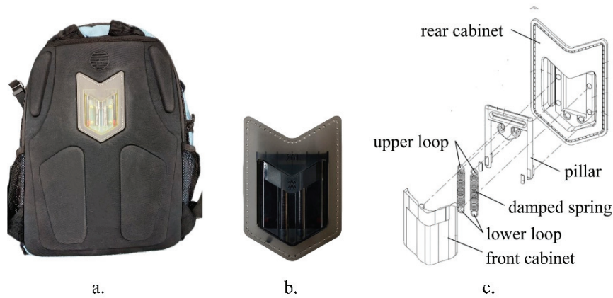
Fig. 1. Schematic of the spring-loaded shock-absorbing backpack design: (a) exterior view of the backpack featuring the integrated protective panel, (b) shock-absorbing device used within the backpack panel, (c) exploded schematic diagram of the shock-absorbing device, showing its structural components, including the front and rear cabinets, damped spring, and connecting loops
