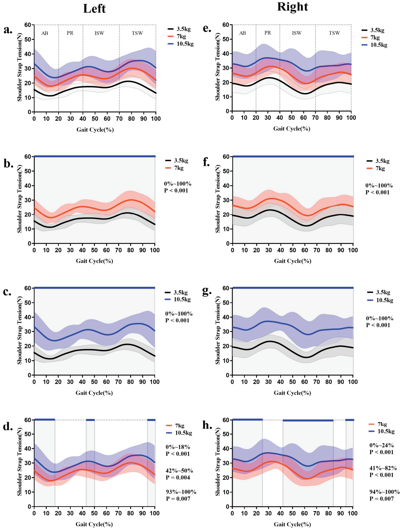
Fig. 4. Shoulder strap tension during the gait cycle for running: AB – absorption, PR – propulsion, ISW – initial swing, TSW – terminal swing
