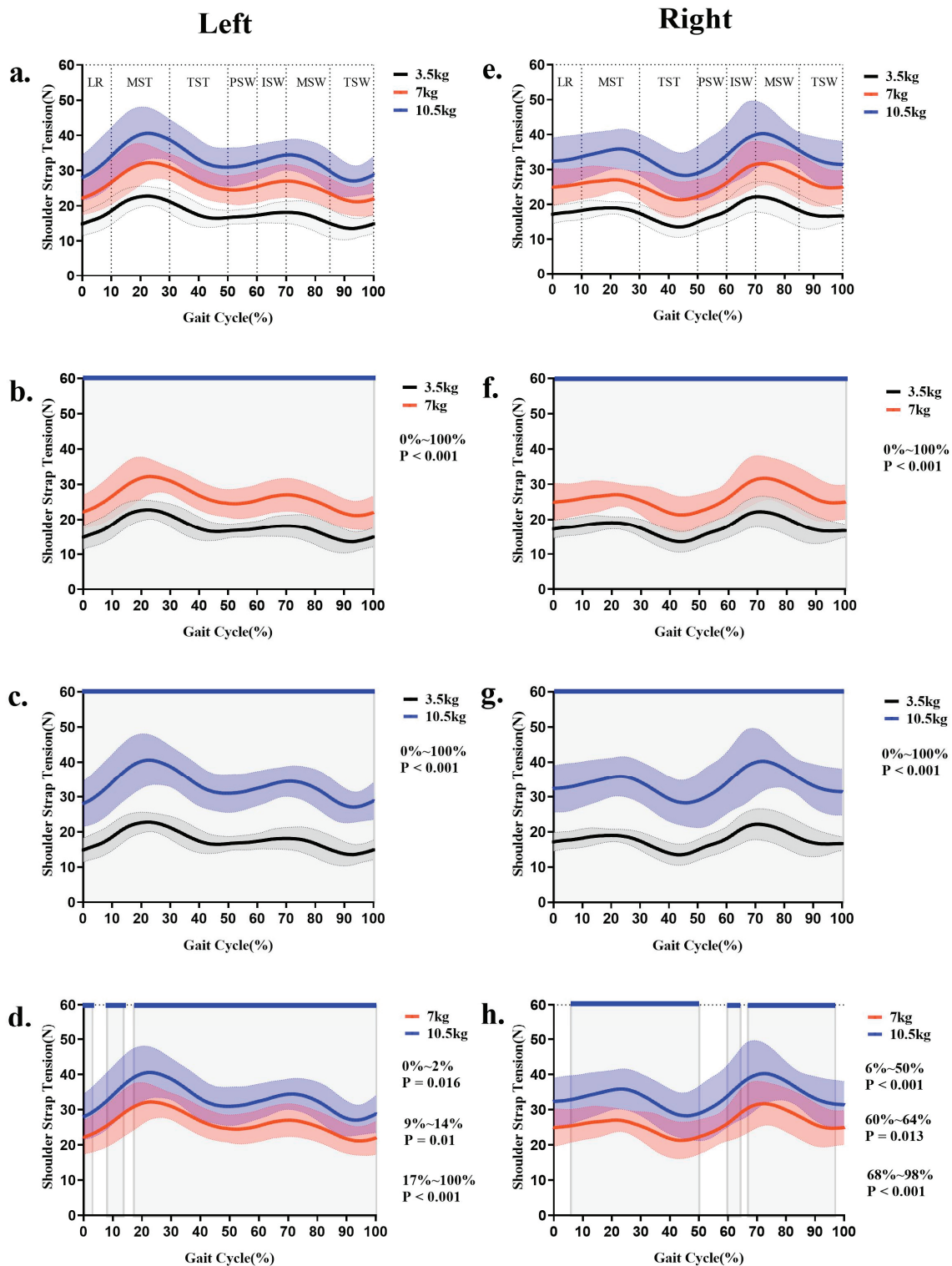
Fig. 3. Shoulder strap tension during the gait cycle for walking: LR – loading response, MST – midstance, TST – terminal stance, PSW – preswing, ISW – initial swing, MSW – midswing, TSW – terminal swing
