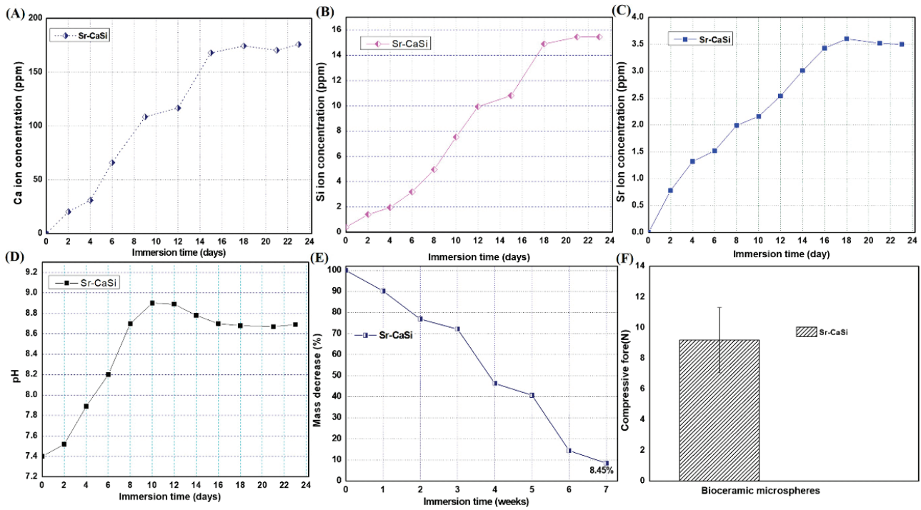
Fig. 3. (A)–(C) in vitro biodissolution test for the bioceramic granules in Tris buffer solution, (D) changes in pH values within 24 days, (E) Mass loss during 7 weeks of immersion, (F) Compressive force for crushing the granule
