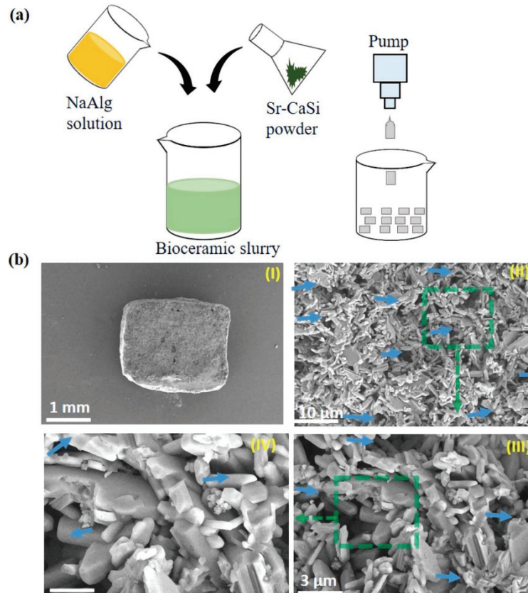
Fig. 2. (a) schematic illustration of the preparation of the granule slurry, (b) SEM micrographs of the granules, blue arrows showing the micropores
