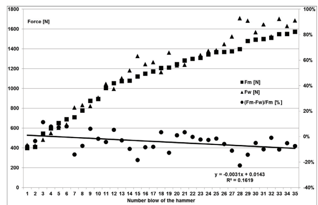
Fig. 6. Graph showing maximal values of the force of test strikes as a function of subsequent strikes; F_m – force of impact of the hammer, F_w – force measured with BTS-4AP-2K
