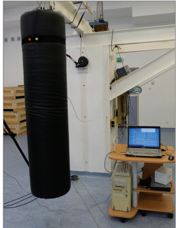
Fig. 1. BTS-4AP-2K dynamometric punching bag with an embedded accelerometer
