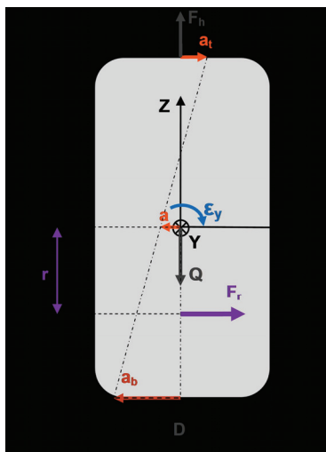
Fig. 3. A simplified, two-dimensional diagram of measured accelerations and forces acting on the dynamometric punching bag having an embedded accelerometer.
