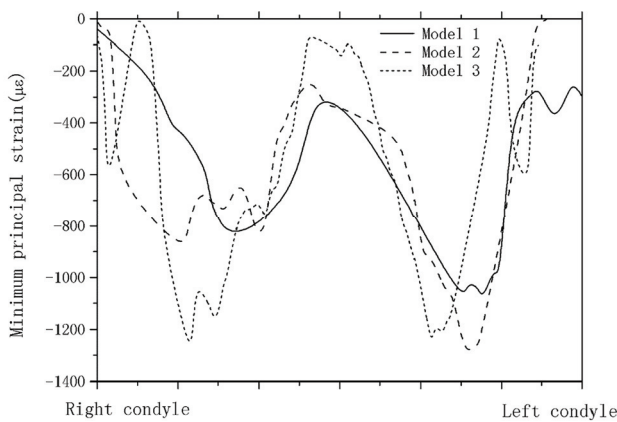
Fig. 12. The minimum principal strains on the external surface of the mandible along the line 2 in 3 models
