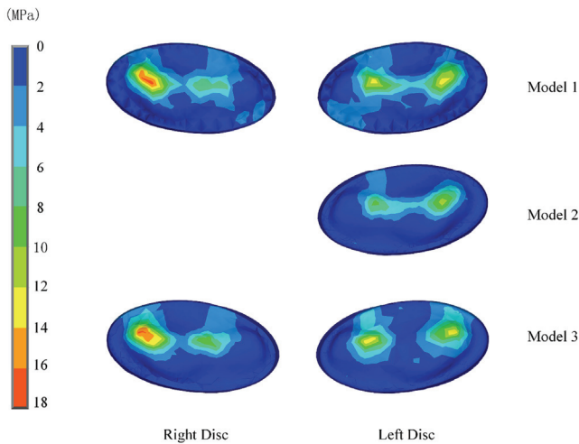
Fig. 4. Von Mises stress distributions of five discs
