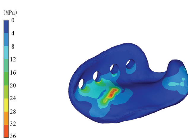
Fig. 5. Von Mises stress distribution of the fossa component of the TMJ prosthesis replacing the right TMJ in Model 2
