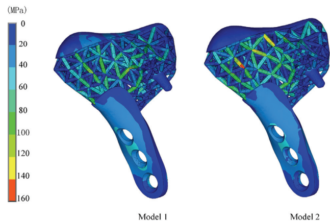
Fig. 6. Von Mises stress distributions of the condyle prosthesis in Model 1 and the condyle component of the TMJ prosthesis in Model 2
