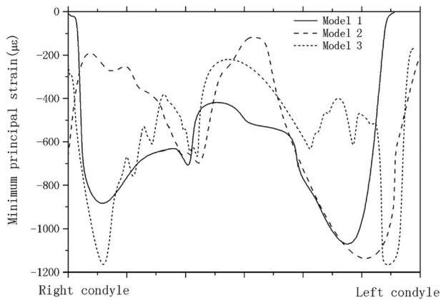
Fig. 11. The minimum principal strains on the external surface of the mandible along the line 1 in 3 models
