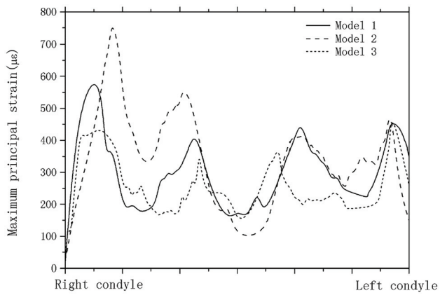
Fig. 9. The maximum principal strains on the external surface of the mandible along the line 1 in 3 models
