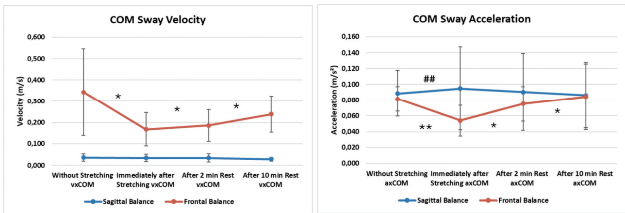
Fig. 2. Center of mass (COM) sway velocity and acceleration:
