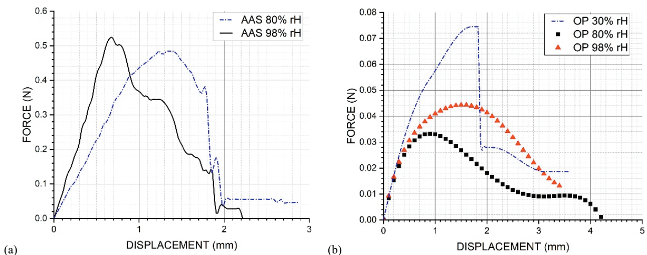
Fig. 6. Example graphs of the force and displacement in various humidity conditions: (a) Attacus atlas , (b) Libellula depressa
