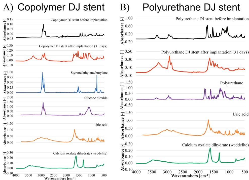
Fig. 2. FTIR spectra of a DJ stent made of styrene/ethylene/butylene block copolymer, and polyurethane, implanted for 31 days
