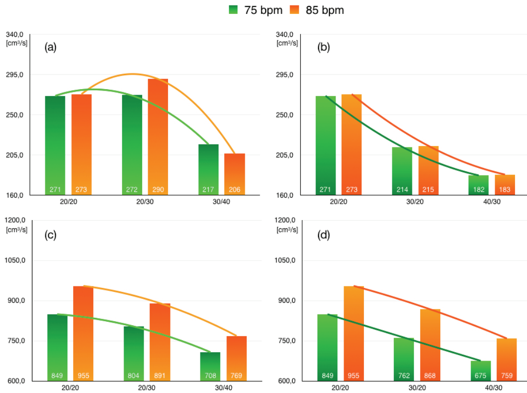
Fig. 5. The change of flows Q_{li} (a), (b) [ \text{cm}^3/\text{s} ] and Q_{lo} (c), (d) [ \text{cm}^3/\text{s} ] at high stenosis of the atrial valve (a), (c) [ \text{g}\cdot\text{s}/\text{cm}^4 ] and at a reverse clinical situation – an increase in mitral valve resistance (b), (d) [ \text{g}\cdot\text{s}/\text{cm}^4 ]
