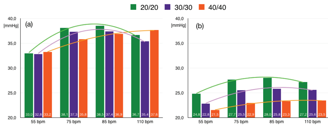
Fig. 6. The change of pressures P_{lv} (a) [mmHg] and P_{cas} (b) [mmHg] at the same level of stenosis of the atrial and mitral valves [ \text{g}\cdot\text{s}/\text{cm}^4 ]
