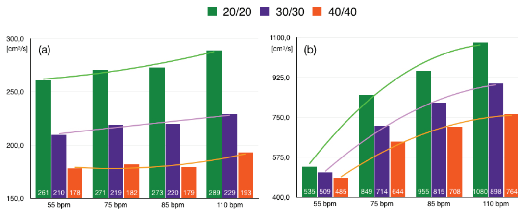
Fig. 7. The change of flows Q_{li} (a) [ \text{cm}^3/\text{s} ] and Q_{lo} (b) [ \text{cm}^3/\text{s} ] at the same level of stenosis of the atrial and mitral valves [ \text{g}\cdot\text{s}/\text{cm}^4 ]
