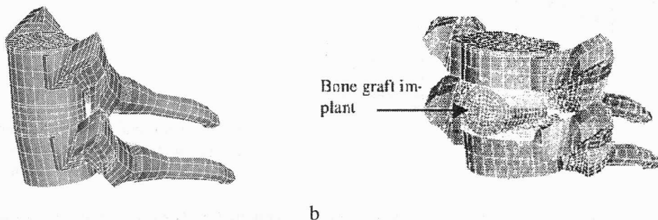
Fig. 2. Finite element mesh for the models: a) intact C5-C6 vertebrae, b) C5-C6 vertebrae after application of the Cloward surgical operation technique
