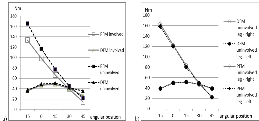
Fig. 2. IT values of PFM and DFM depending on the angle of foot positioning towards the shin in group I (a) and group II (b)
