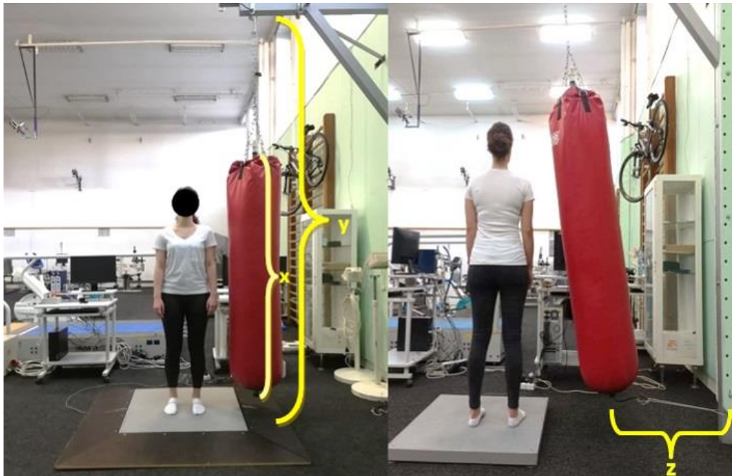
Figure 1. The participant's position on the platform, where: x – the length of the punchbag, y – the height from the attachment to the ground, z – distance between wall and the middle of the boxing bag.
