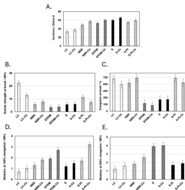
Figure 2. Mechanical properties: Shore A hardness (A), tensile strength (B), elongation at break (C), Young's modulus at 100% elongation (D) and Young's modulus at 200% elongation (E) of LC, LC-Ch, NBR, NBR-Ch, EPDM, EPDM-Ch, S, S-Ch, S-Pt, and S-Pt-Ch rubber materials.
