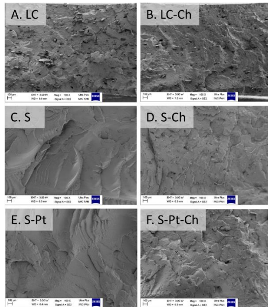
Figure 1. SEM images for LC (A), LC-Ch (B), S (C), S-Ch (D), S-Pt (E), S-Pt-Ch (F).
