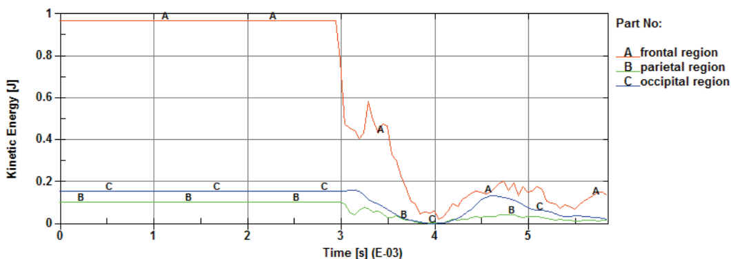
Fig. 6. Kinetic energy in bridging veins as a function of time A – frontal region; B – parietal region; C – occipital region under impact loading in the range of 3–4 ms
