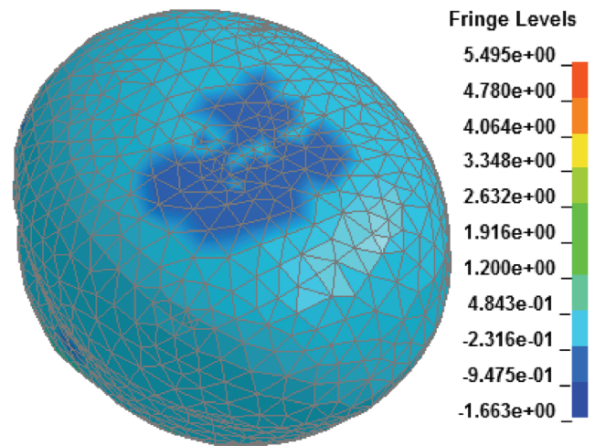
Fig. 12. Principal stress 1st in dura mater. Max stress 5.50 MPa
