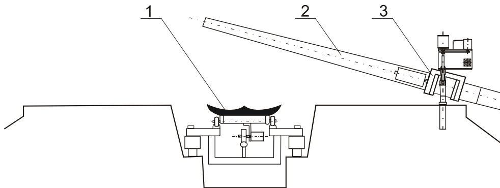
Fig. 4. Schematic diagram of the pool station for the measurement of biomechanical parameters of rowing: 1 – sliding seat with motion sensor, 2 – measuring oar with strain gauge, 3 – measuring oarlock attached to the oar
