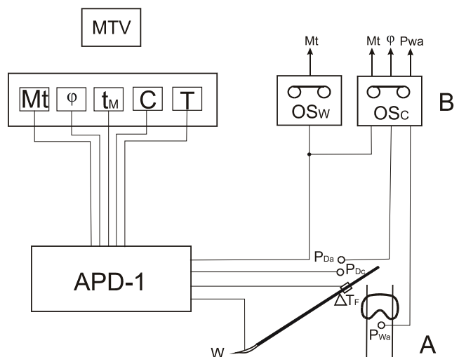
Fig. 6. Schematic of the Rowing Pool Testing Station BTW-1
