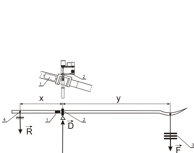
Fig. 5. Illustration of the strain gauge calibrating procedure used for the measurement of driving forces (torques) acting on the oar: 1 – strain gauge, 2 – oarlock, 3 – calibration weights ( F ), D – reaction force on oarlock, R – reaction force on oar blocking system
