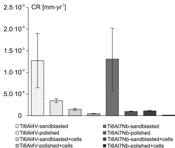
Fig. 3. Corrosion rate of titanium alloys in PBS
